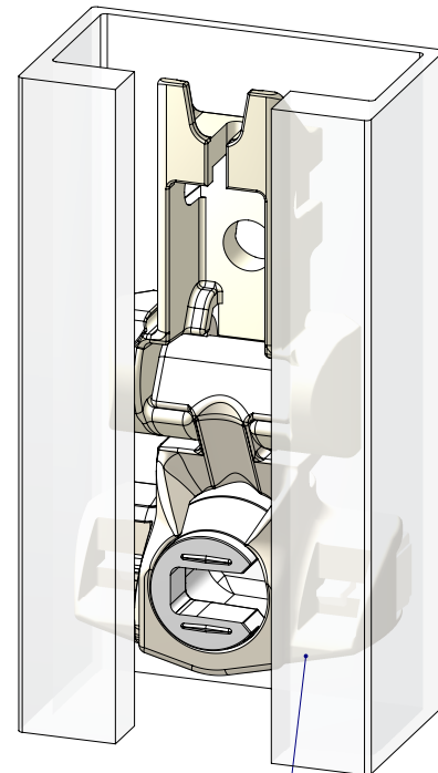
CARRIER ASSEMBLY, 20B0013 (.562"x1.292")
