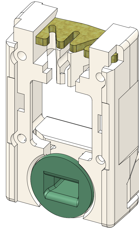
Carrier Assembly 16H82 (Unlocked Position)
