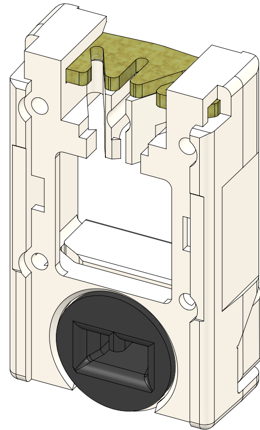
Carrier Assembly 16H70 (Unlocked Position)
