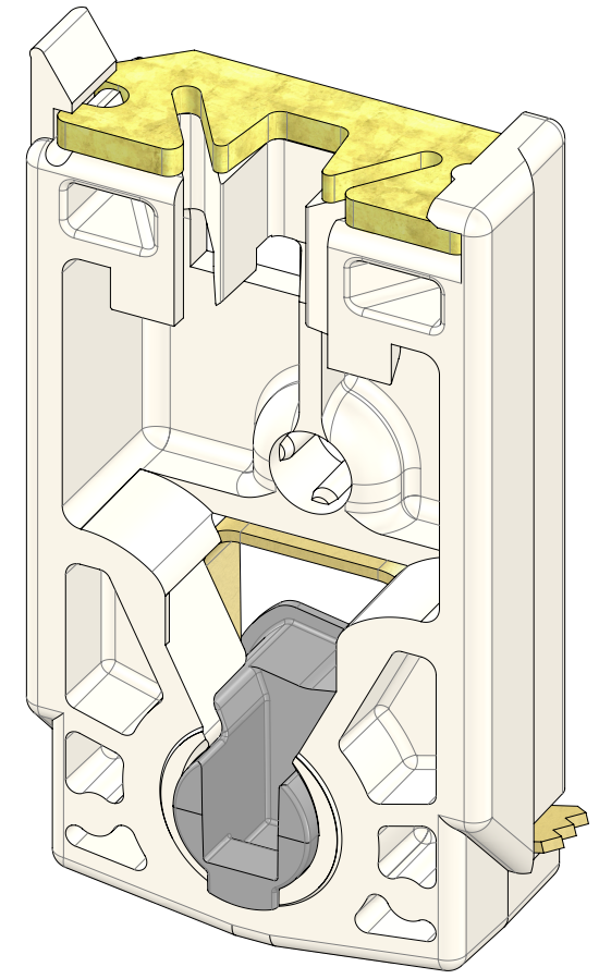
.562 Carrier Assembly 15B111 (Locked Position)
