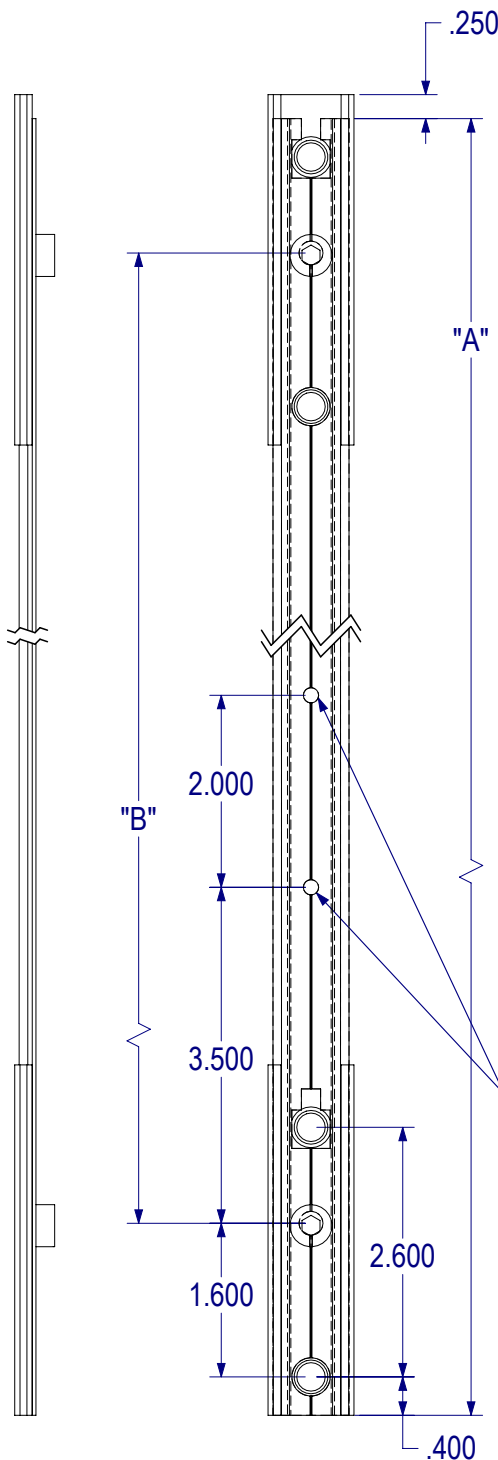
8311 Offset Drive Lock Bar
