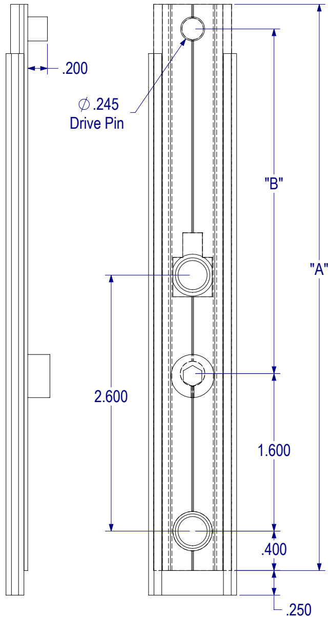
8300B Single Point Below Handle Lock Bar
