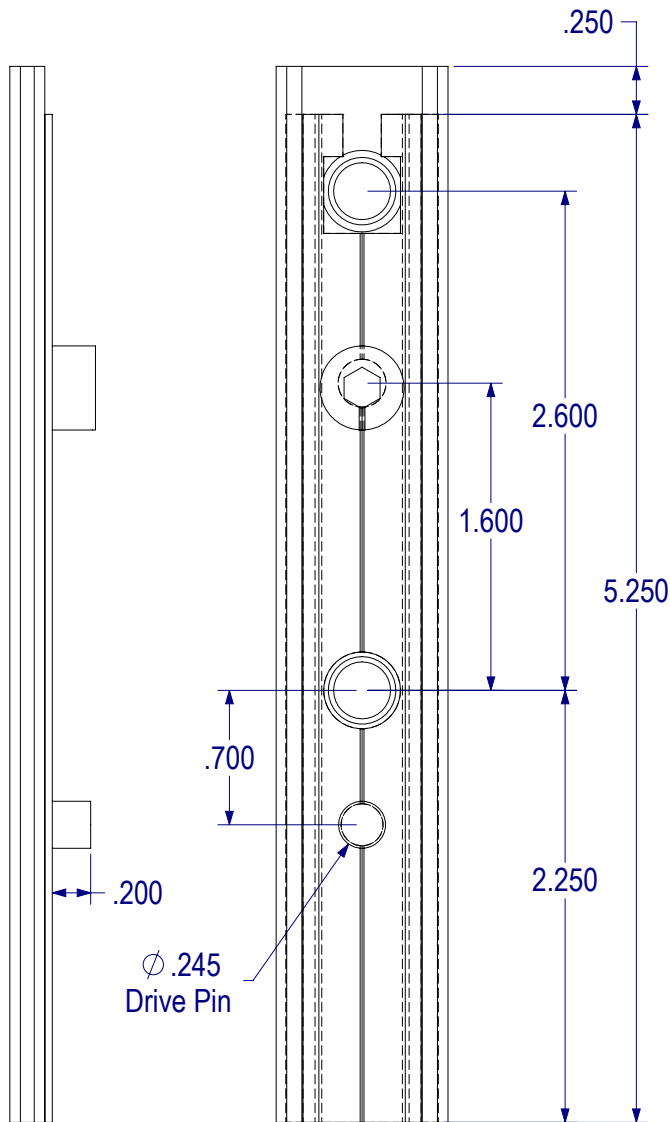
8300-5.25 Single Point Above Handle Lock Bar
